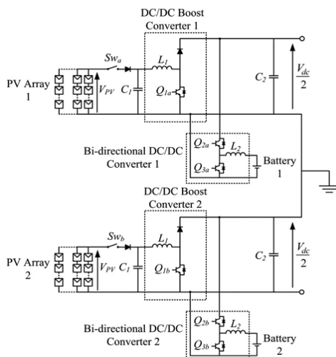
Figure 7: Proposed PV battery system
