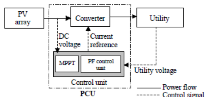
Figure 5: Schematic diagram of Grid connected PV system
