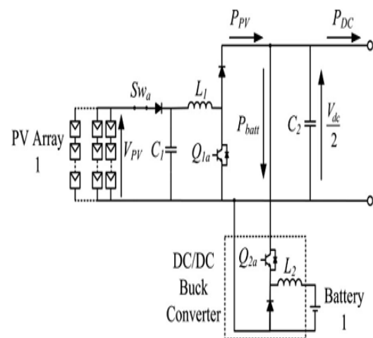
Figure 8: Circuit during charging operation
