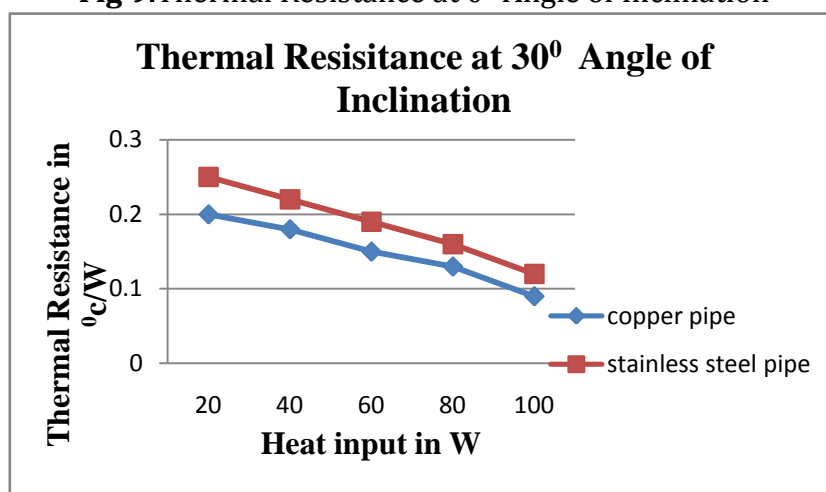
Fig 10. Thermal Resistance at 30° Angle of Inclination
