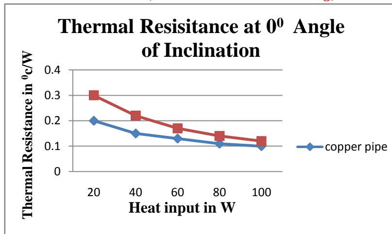
Fig 9. Thermal Resistance at 0° Angle of Inclination
