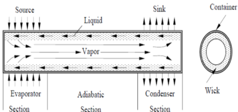
Fig.1 Heat Pipe
