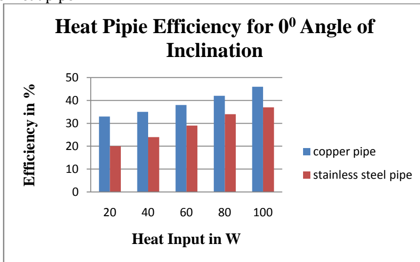
Fig 12. Heat Pipe Thermal Efficiency for 0 0 Angle of Inclination
