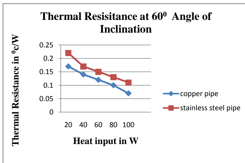
Fig 11. Thermal Resistance at 60° Angle of Inclination
