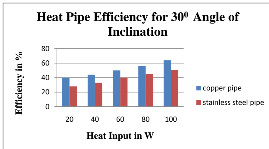
Fig 13. Heat Pipe Thermal Efficiency for 30 0 Angle of Inclination
