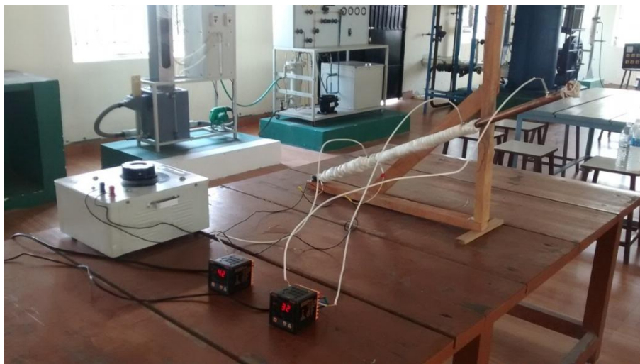
Fig. 7 Heat Pipe at 30^\circ Angle of Inclination
