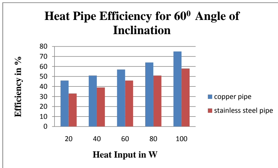
Fig 14. Heat Pipe Thermal Efficiency for 60° Angle of Inclination
